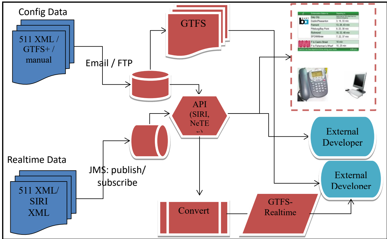
Figure 1 – Transit data communication architecture for San Francisco Bay Area 511
